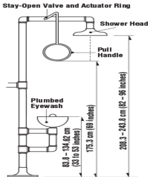
Fig.1 Shower Station
